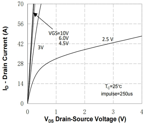
Figure 1. On-Region Characteristics
