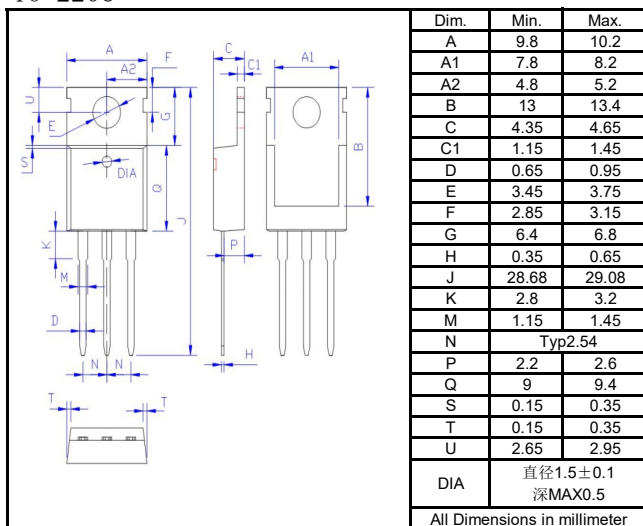
TO-220C
